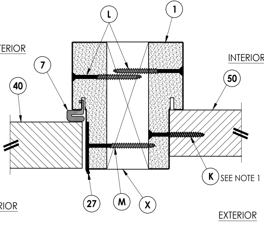
5 6 HORIZONTAL CROSS SECTION Outswing
