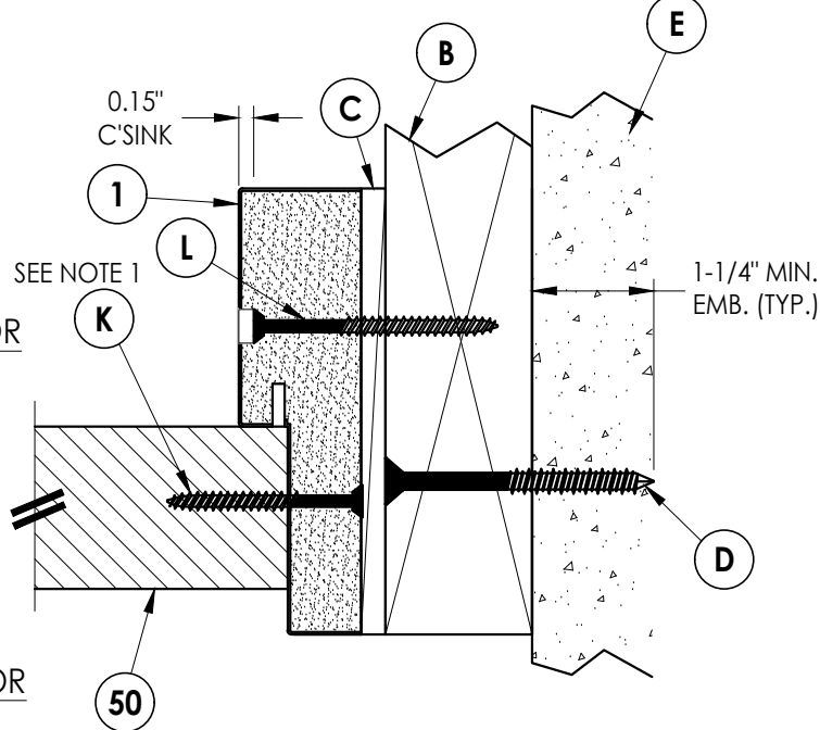
6 6 HORIZONTAL CROSS SECTION Outswing 2X Buck Construction
