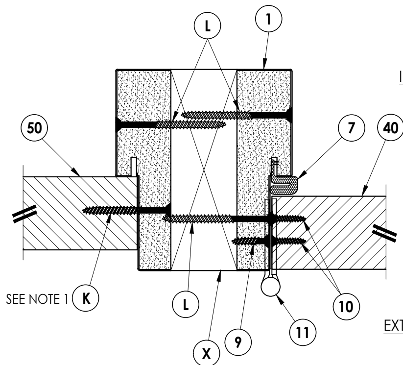
4 6 HORIZONTAL CROSS SECTION Outswing
