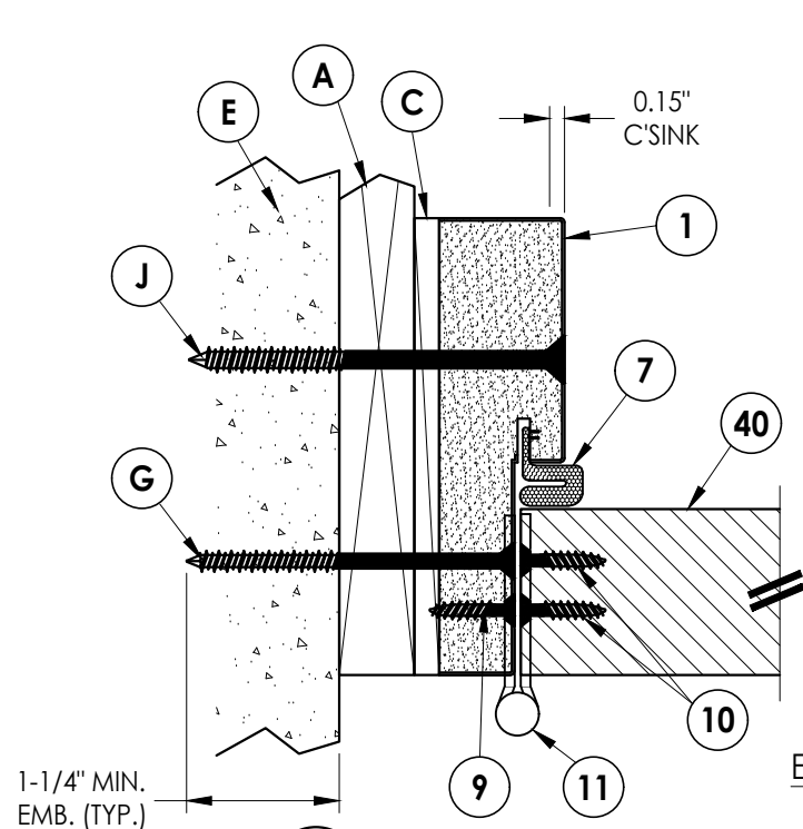
3 6 HORIZONTAL CROSS SECTION Outswing 1X Buck Construction
