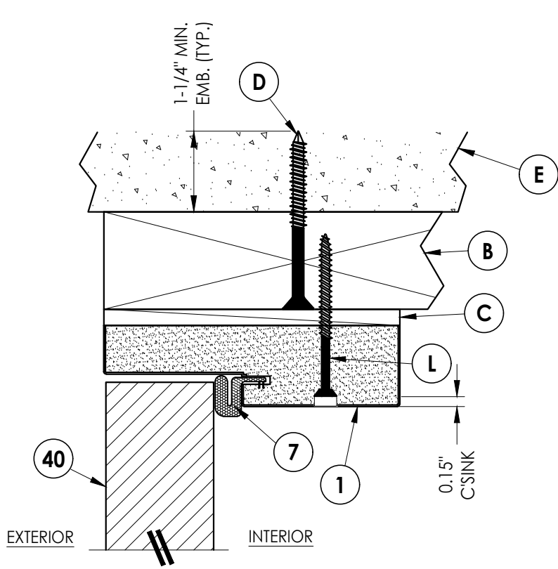
1 5 VERTICAL CROSS SECTION Outswing 2X Buck Construction
