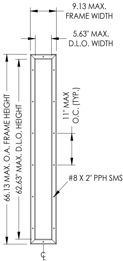
ODL LITE FRAME 14" SIDELITE PANEL
