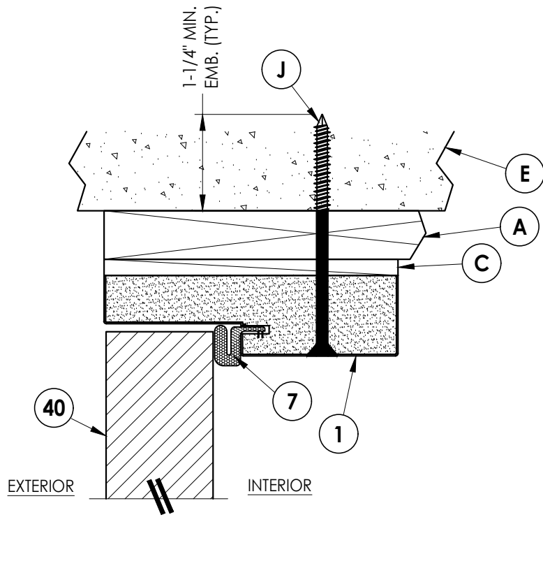
2 5 VERTICAL CROSS SECTION Outswing 1X Buck Construction
