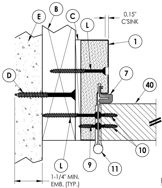
1 6 HORIZONTAL CROSS SECTION Outswing 2X Buck Construction
