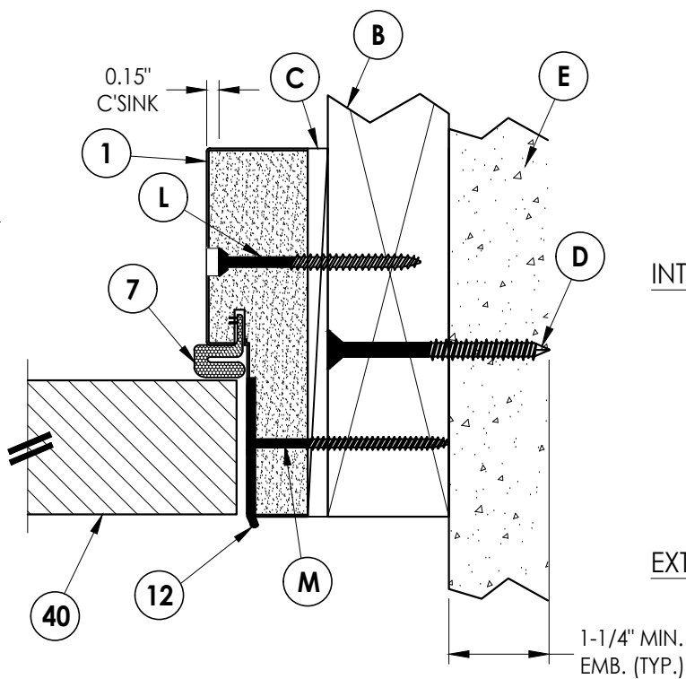
2 6 HORIZONTAL CROSS SECTION Outswing 2X Buck Construction
