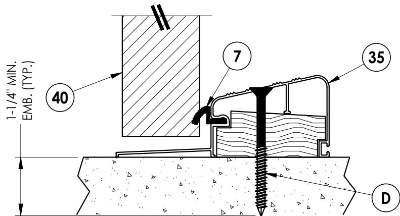
4 5 VERTICAL CROSS SECTION Outswing Bump Threshold
