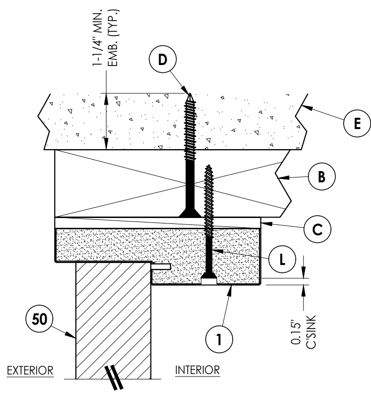
3 5 VERTICAL CROSS SECTION Outswing 2X Buck Construction
