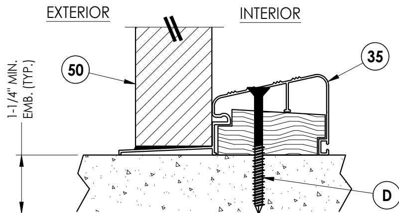
5 5 VERTICAL CROSS SECTION Outswing Sidelite Threshold
